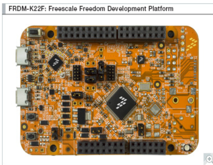
Figure 1. FRDM-K22F top view
